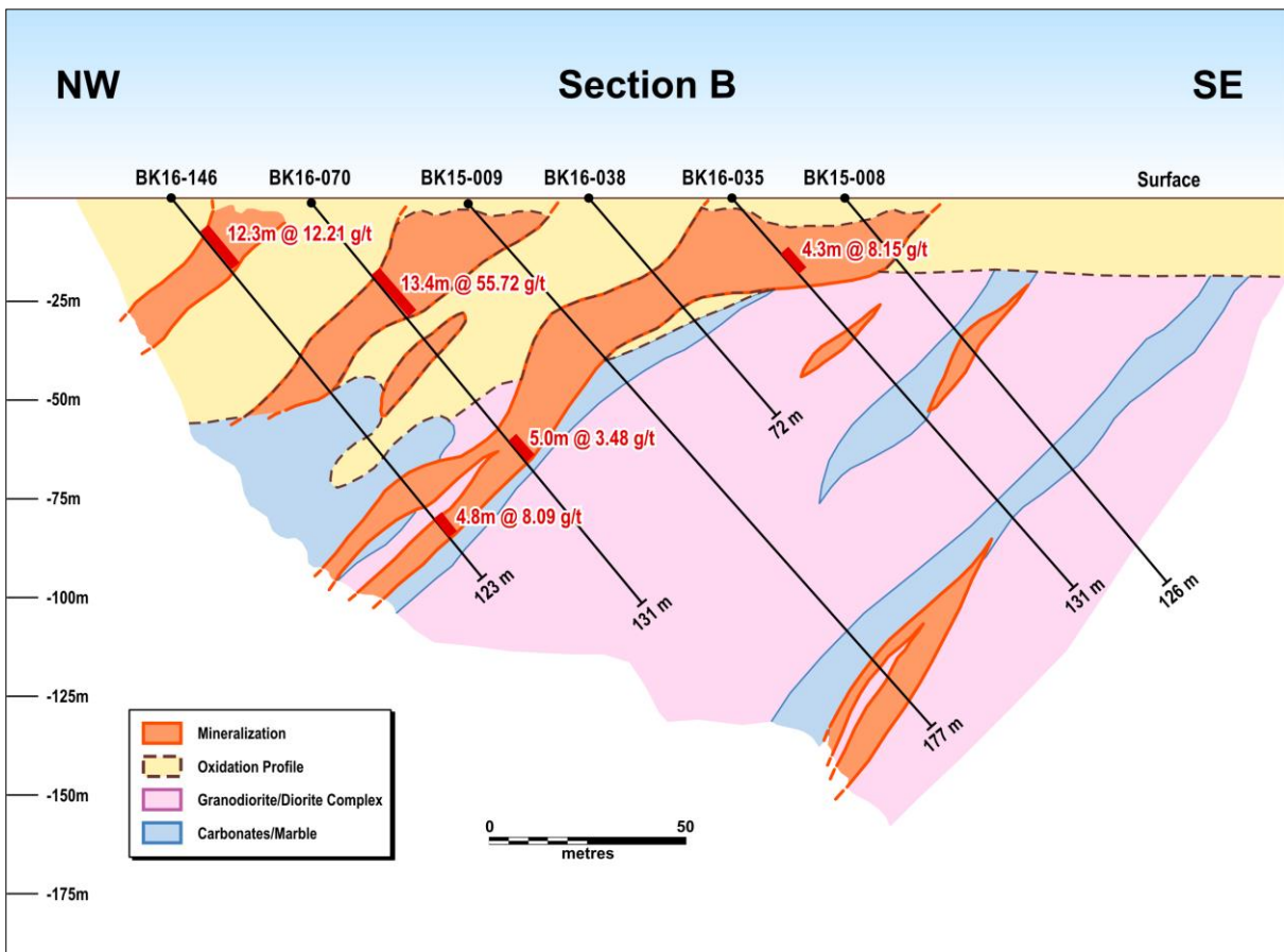
Figure 4: Cross-Section B
