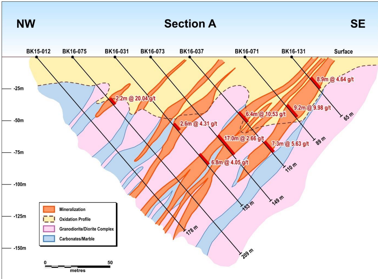
Figure 3: Cross-Section A
