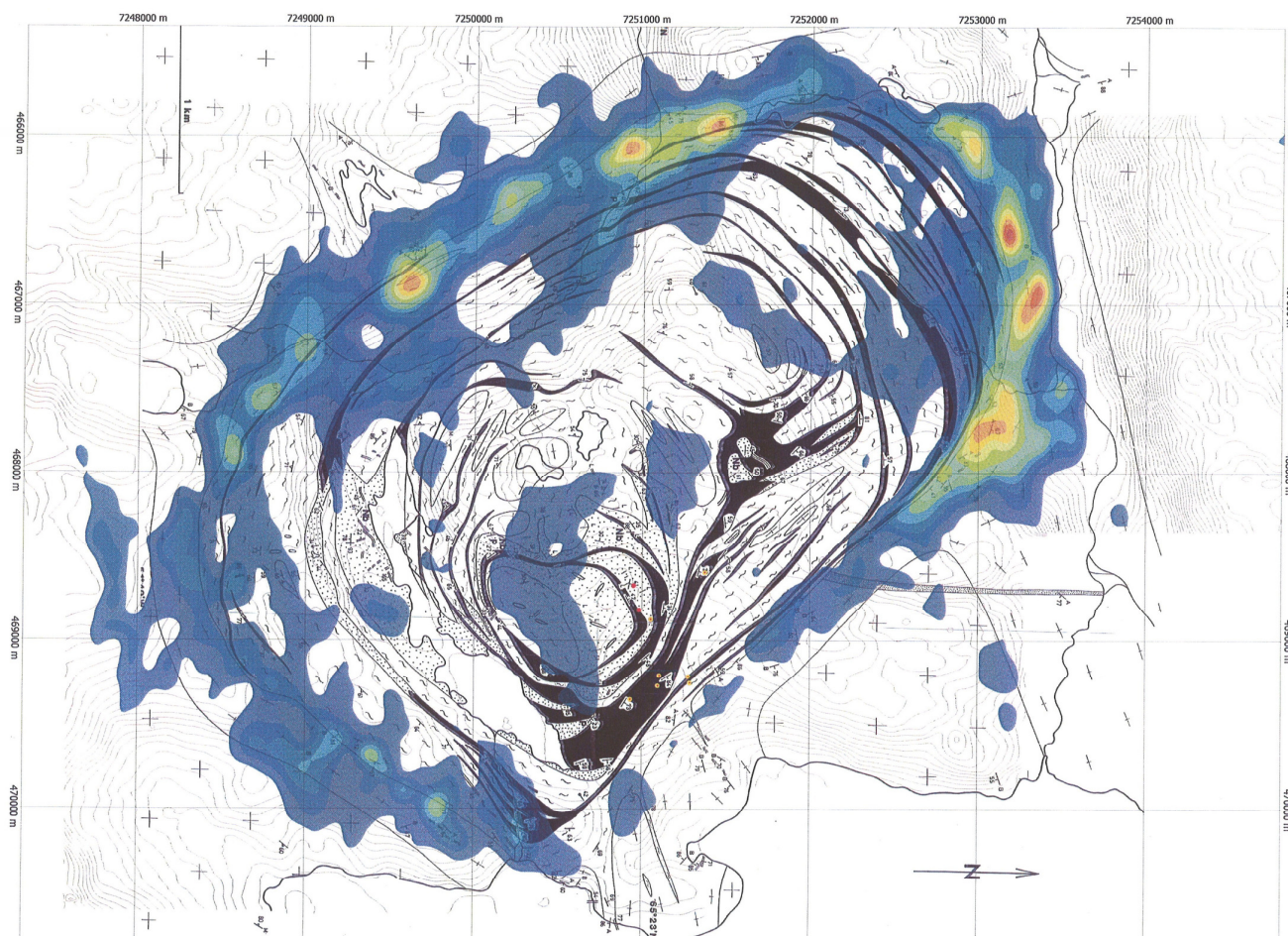
QEQRITAASAQ: Shaded contours depicting thorium radiometric survey flown in 2000 are superimposed on a geological map by GEUS published in 1987. Grid blocks are 1000 m.
