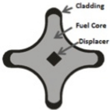
Standard Uranium Oxide and Lightbridge Metallic Fuel Rod Cross Sections
