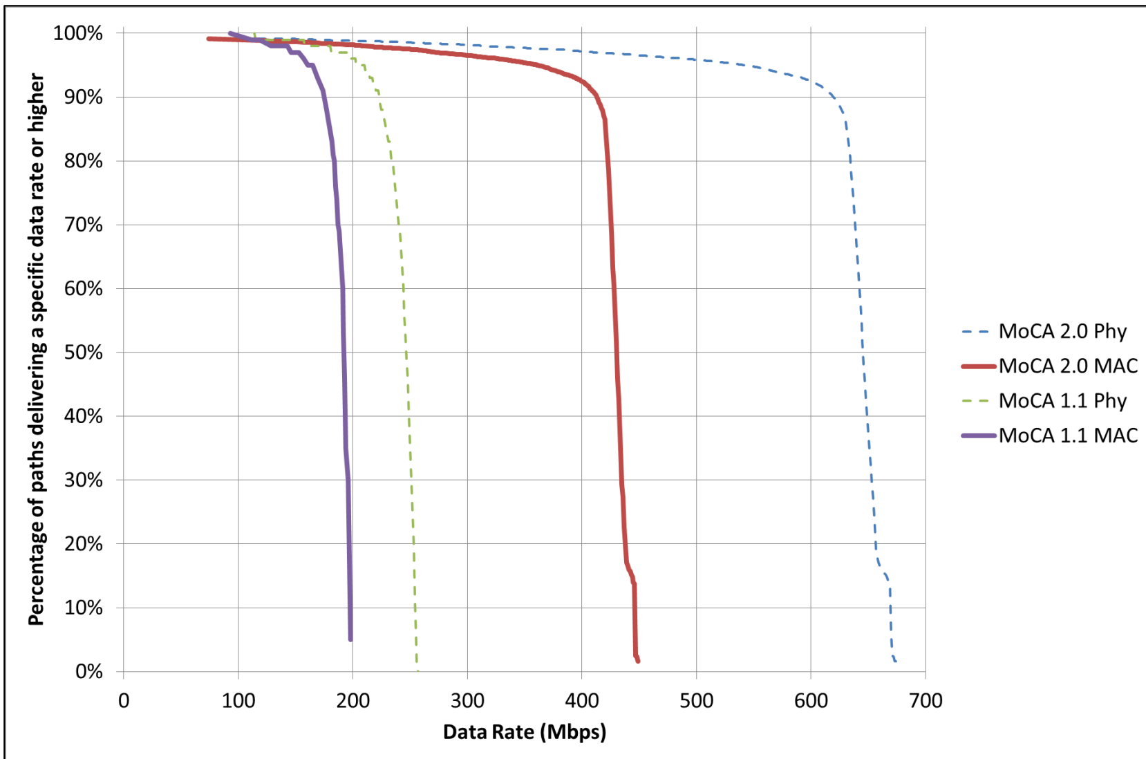
Chart shows the percentage of paths delivering a specific data rate or higher for both raw data (PHY) and net (MAC) throughput. ©2015 Multimedia over Coax Alliance
